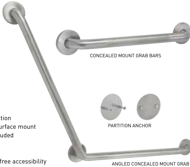
ANGLED CONCEALED MOUNT GRAB BAR
