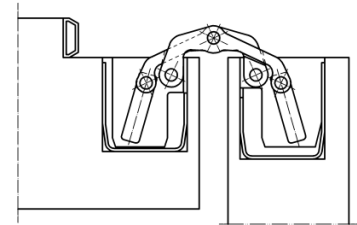
Blockzarge 180°
