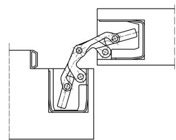
Blockzarge 90°
