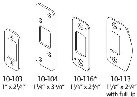
Standard door prep for B-Series installation.
