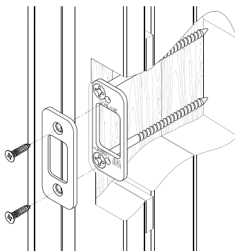
Strike reinforcement plate with 3" screws provides maximum resistance to kick-in attacks.
