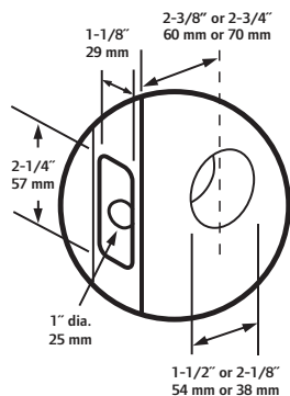
Standard door prep for B-Series installation.
