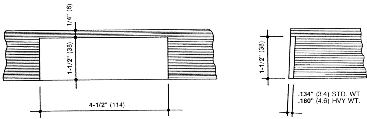
DOOR HINGE CUT-OUT PREPARATION
