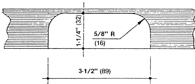
DOOR HINGE CUT-OUT PREPARATION
