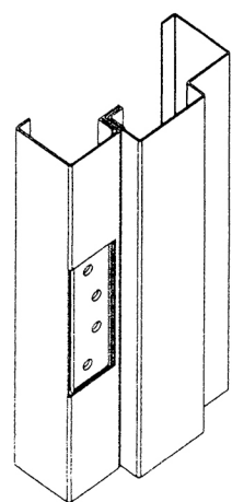
4-1/2" (114) UNIVERSAL HINGE PREPARATION 7Ga. (4.1) REINFORCEMENT WITH DUST BOX FOR STANDARD OR HEAVY WEIGHT HINGES D & T FOR #12-24 SCREW
