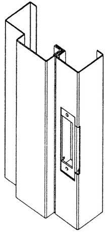
4-7/8" (124) STRIKE PREPARATION [ANSI A155.1] 14 Ga. (2.0) REINFORCEMENT WITH DUST BOX D & T FOR #12-24 SCREW
