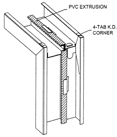
TYPICAL CORNER SECTION
