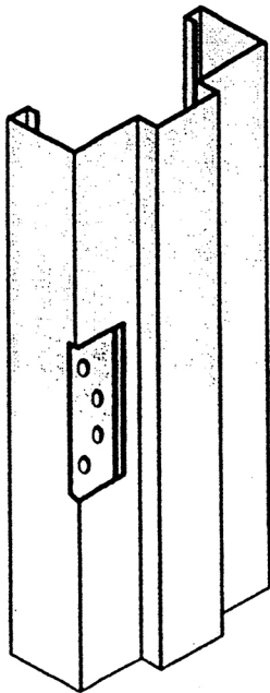
4-1/2" (114) HINGE PREPARATION— 7 GA. (3.4) REINF. WITH DUST BOX
