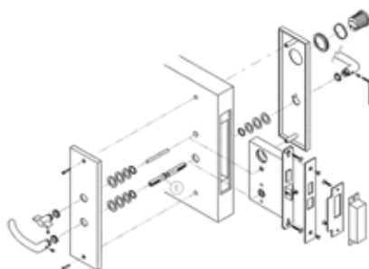
Figure 26 ML F ERS trim
