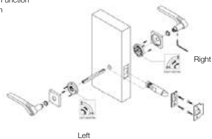
Figure 4 Dummy Trim For rosette and escutcheon
