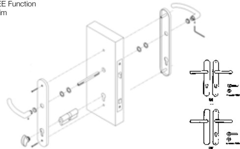
Figure 32 Entry EE Function RSM trim
