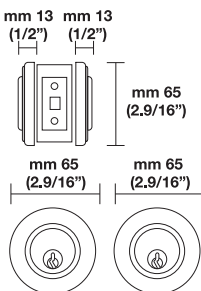
102 DOUBLE CYLINDER
