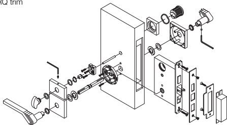
Figure 11 ML F RQ trim
