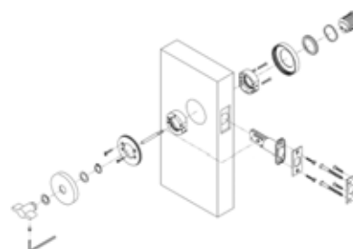
Figure 25 Deadbolt Single Cylinder 101 RPS
