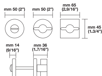
105 PRIVACY BOLT Stainless steel AISI 316 L
