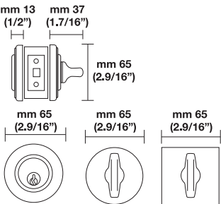
101 SINGLE CYLINDER
