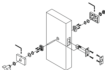
Figure 24 Privacy Bolt 105 RSQS
