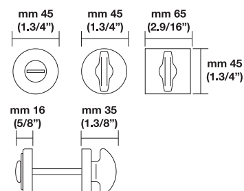
105 PRIVACY BOLT Solid brass
