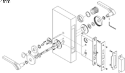
Figure 12 ML F RP trim
