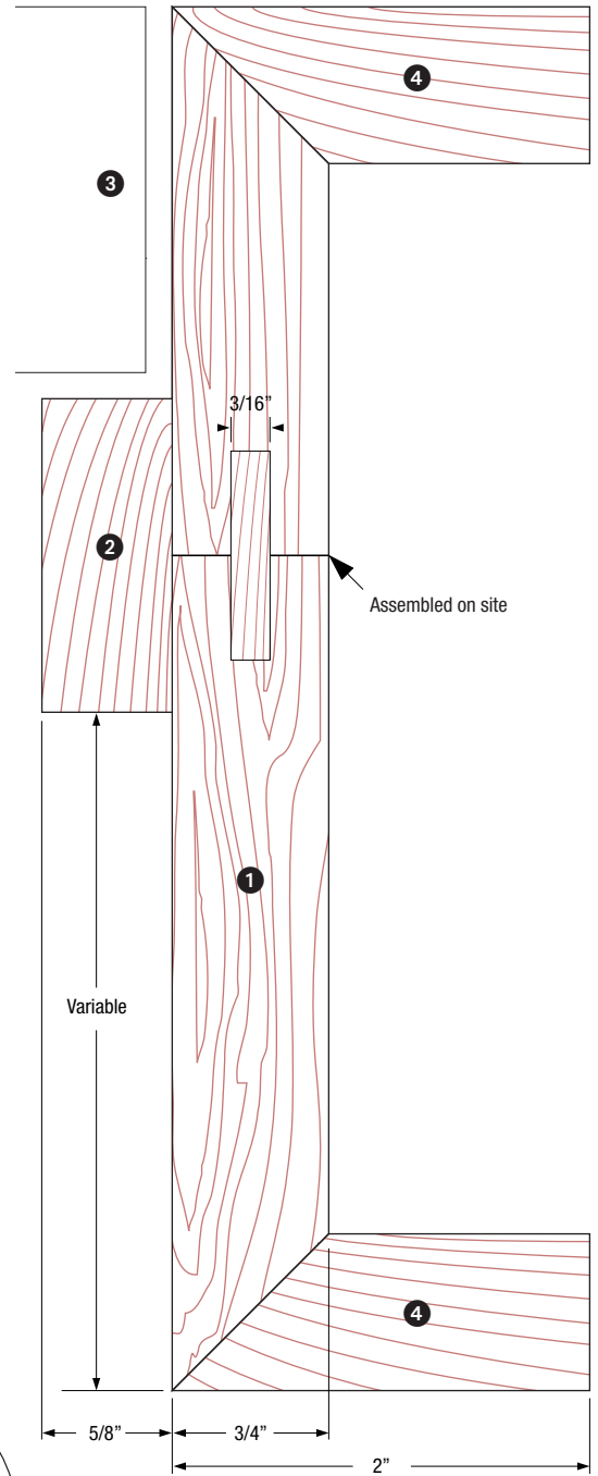
JAMB ASSEMBLY Head and jamb
