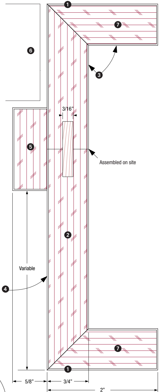
JAMB ASSEMBLY Head and jamb
