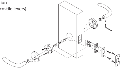
Figure 4 Privacy Function For long escutcheon plates EP trim
