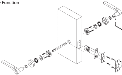
Figure 3 Dummy Trim For rosette and escutcheons
