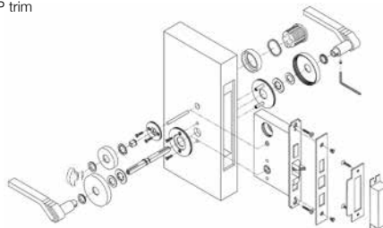
Figure 12 ML F RP trim
