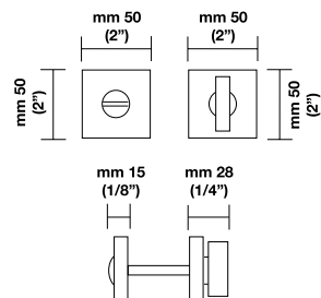
105 RSQ/K 1225 RSQ (2" x 2") Solid brass
