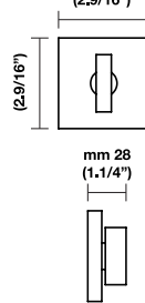
101 RQ / K1225 Solid brass mm 65 (2.9/16")
