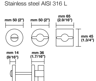
105 PRIVACY BOLT Stainless steel AISI 316 L
