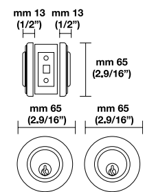
102 DOUBLE CYLINDER
