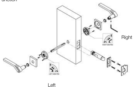
Figure 2 Passage Function RSQ Trim
