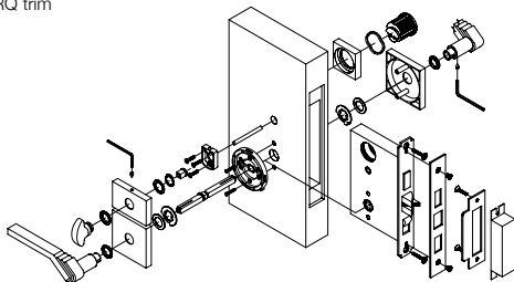
Figure 11 ML F RQ trim
