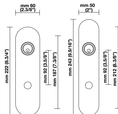
NES Narrow Plain Escutcheon Stainless steel
