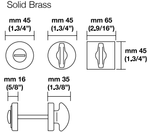
105 PRIVACY BOLT Solid Brass
