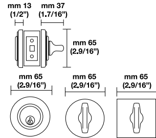
101 SINGLE CYLINDER
