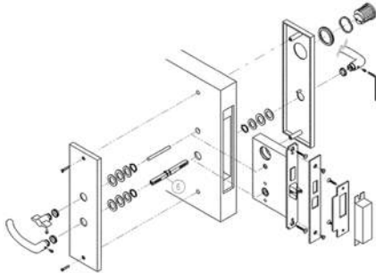
Figure 26 ML F ERS trim
