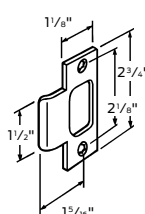
005075-000 T-strike, square corner
