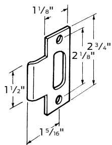
Q001-046 T-strike square corner
