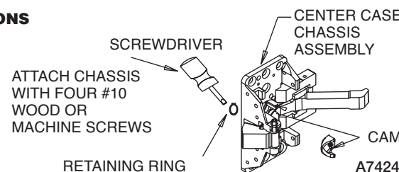
RETAINING RING
